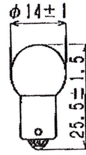
G14 BA9S/13
