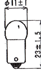
G11B BA9S/13
