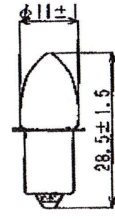
B11 P13.5s/14
