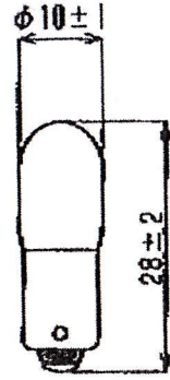
T10B BA9S/13
